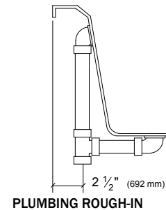
PLUMBING ROUGH-IN
